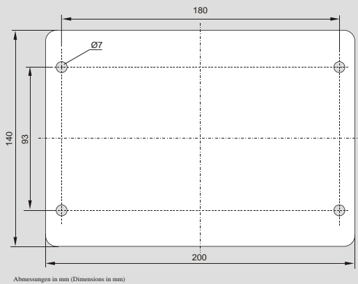
Wandmontage (Wall mounting)
