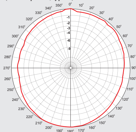
Horizontaldiagramme, horizontale Polarisation: — vertikale Polarisation: — (Horizontal pattern, vertical/horizontal polarised) 192 MHz
