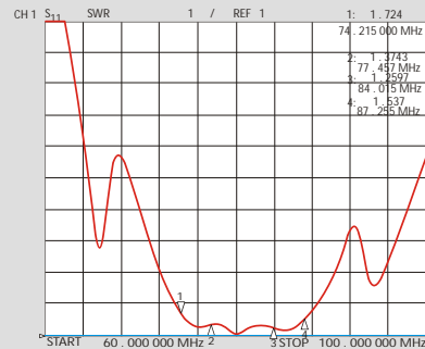
VSWR 4m Band
