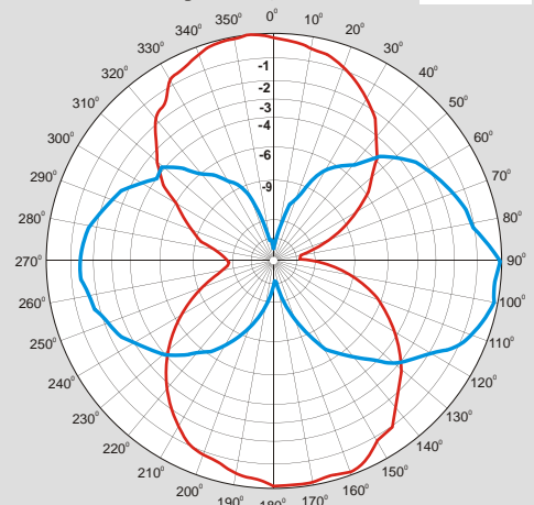
Horizontaldiagramme, horizontale Polarisation: — vertikale Polarisation: — (Horizontal pattern, vertical/horizontal polarised)
